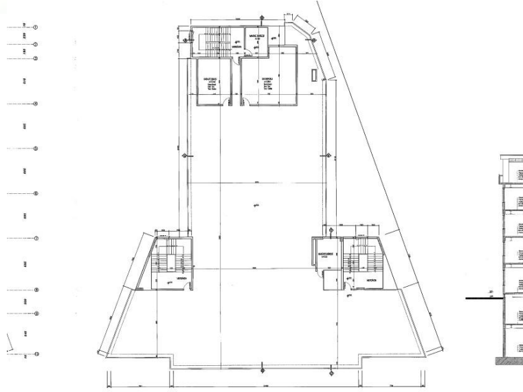
ÇATI PLANI 0:1/100
